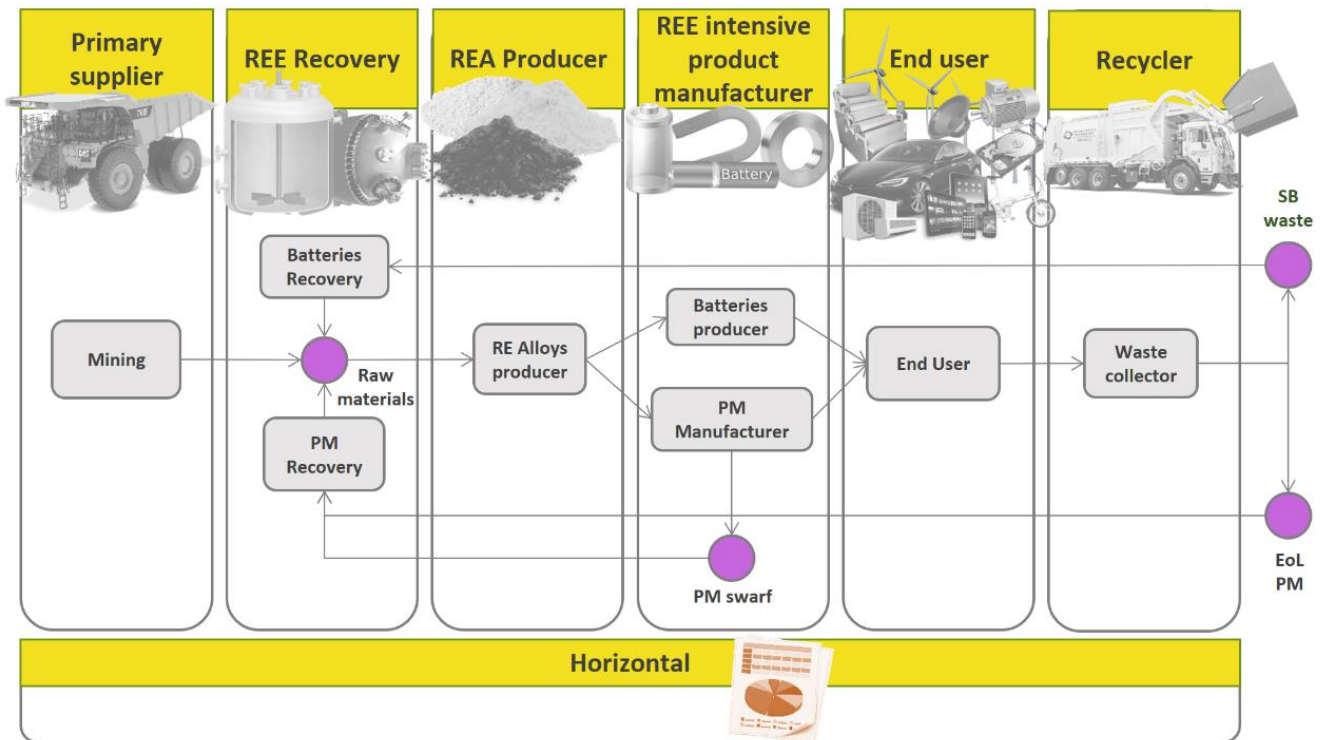
FIGURE 1 THE REE GLOBAL SUPPLY CHAIN SHOWING THE EXAMPLE OF RECOVERY FROM TWO WASTE STREAMS PERMANENT MAGNET SWARF AND BATTERIES.
